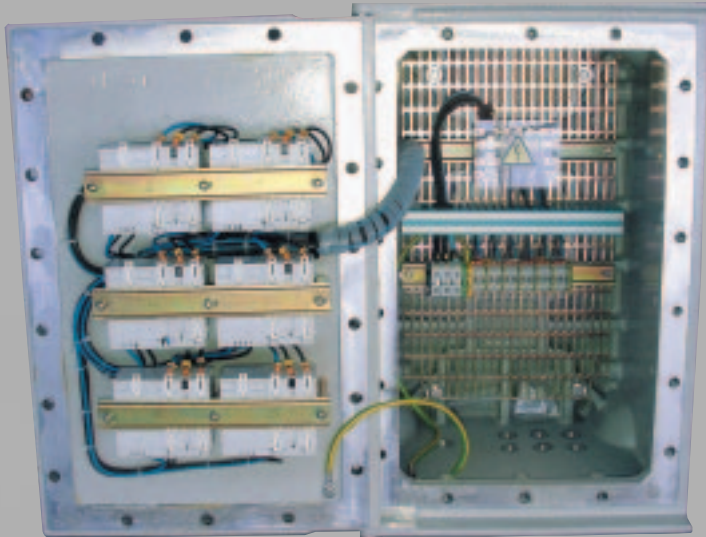
Customised switchboard
